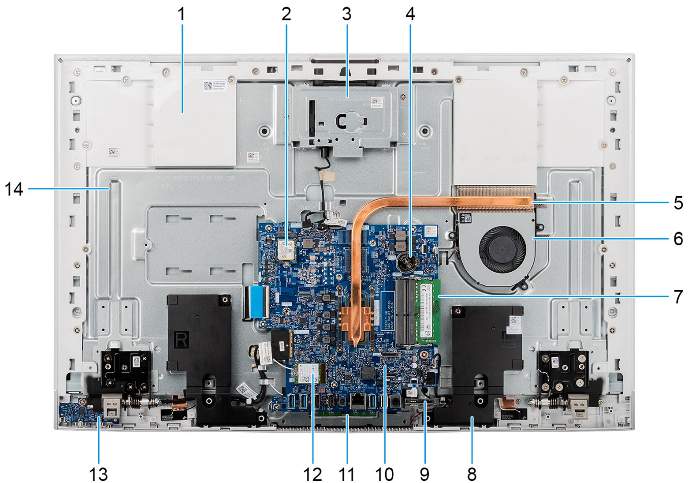
Figure 7. Inside view of your computer
